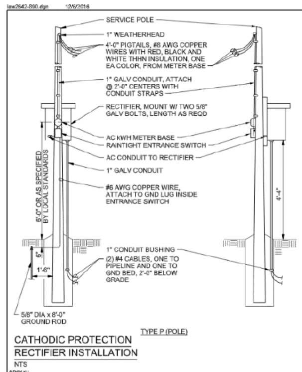
Figure 5. Section showing pole-mounted CPR
