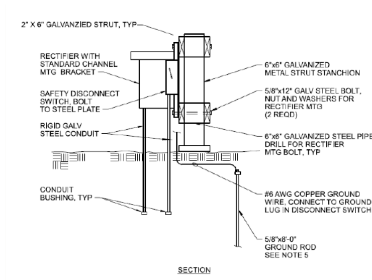
Figure 4. Section showing station-mounted CPR proposed at intertie
