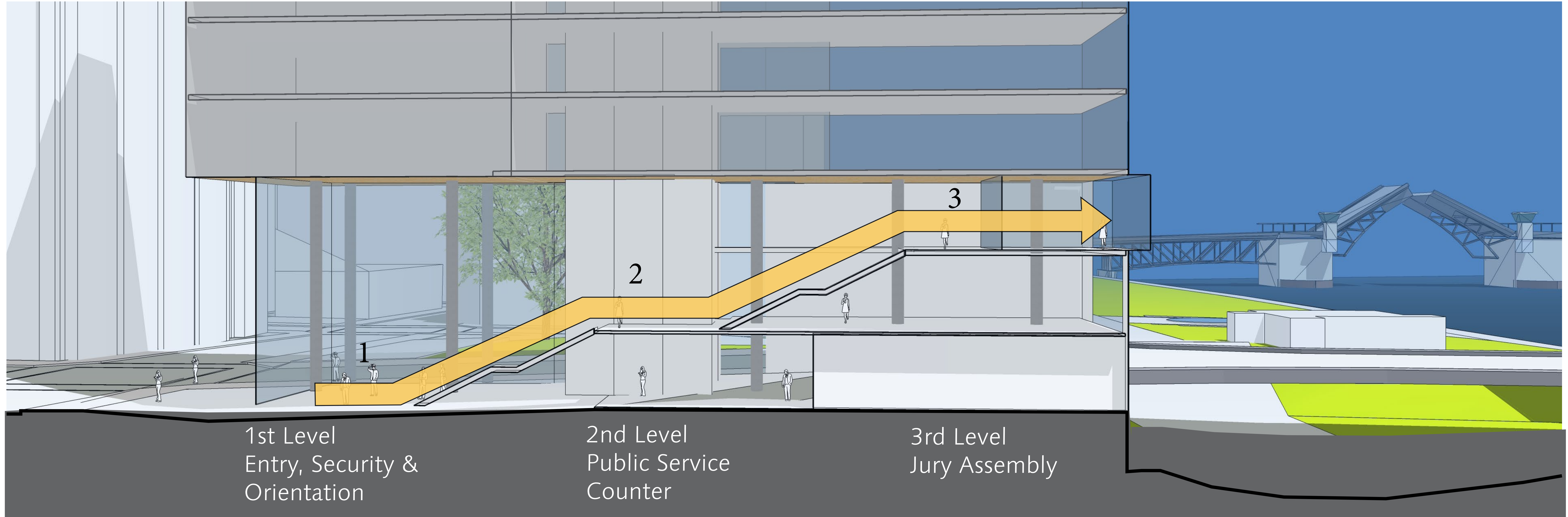
LOBBY SECTION DIAGRAM
